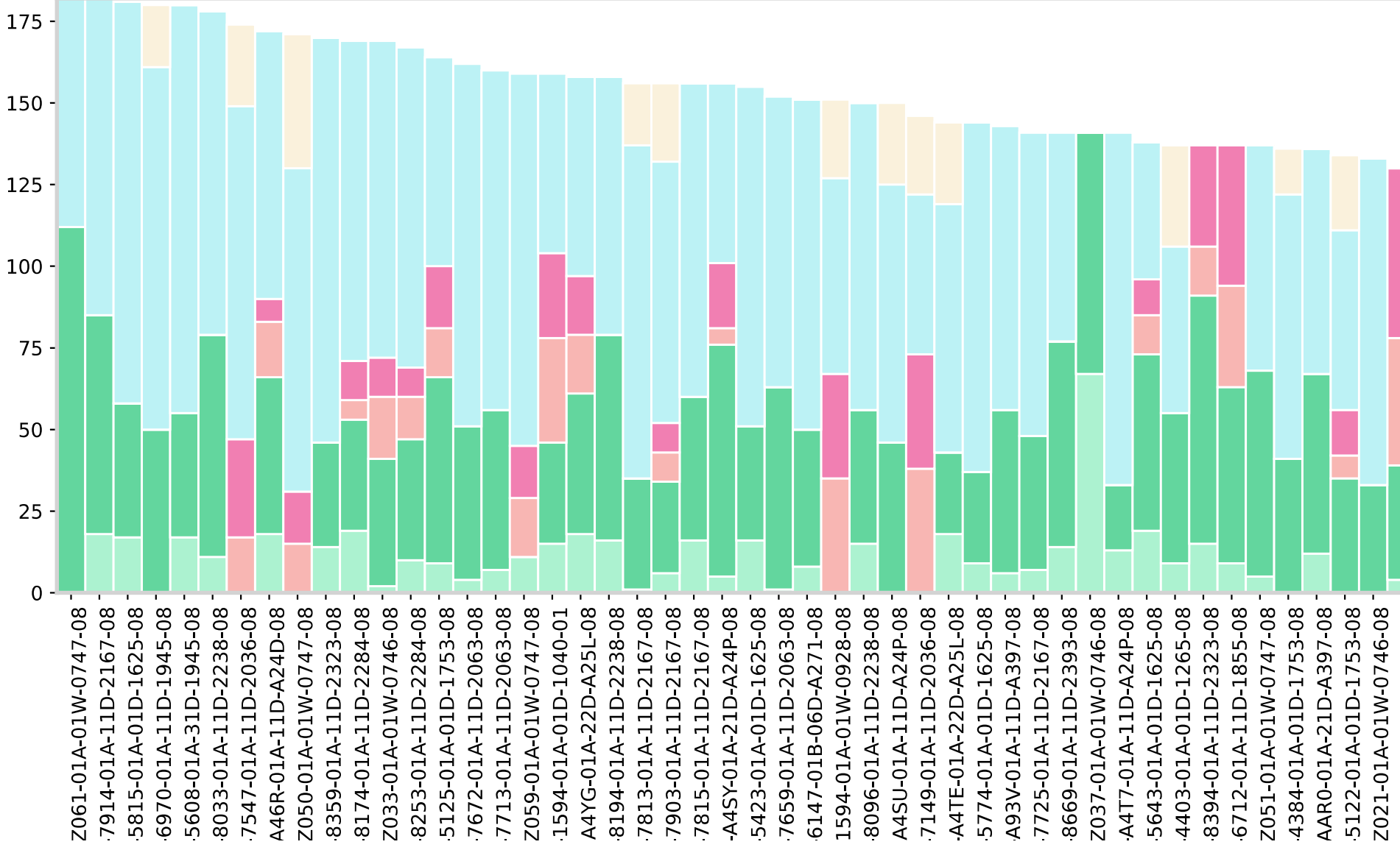
Number of mutations in each signature
